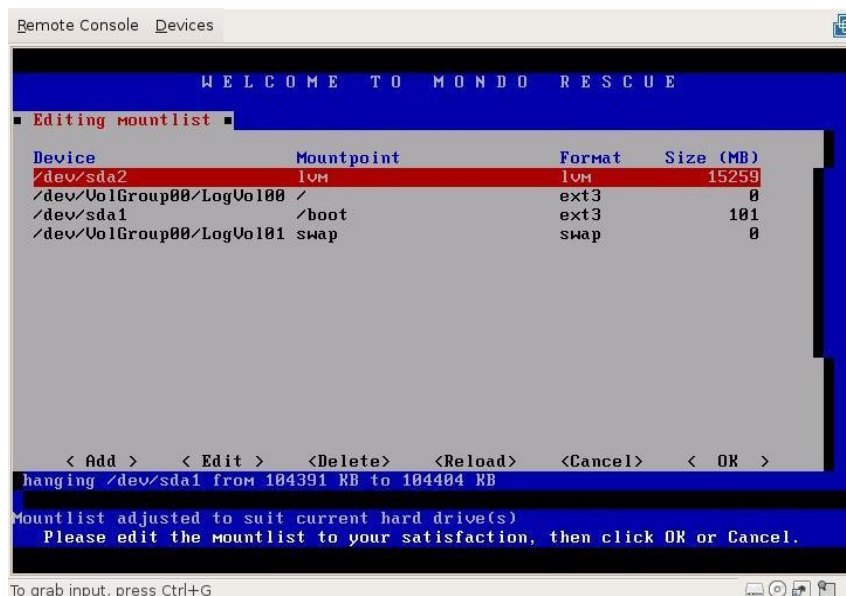
Figure 3: Editing mountpoints
